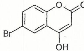
6-Bromo-4-hydroxy coumarin
