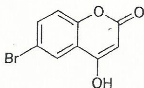
6-Bromo-4-hydroxy coumarin
